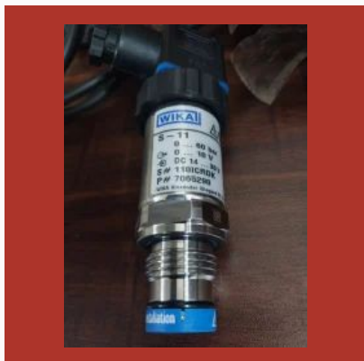
Wika Pressure Transmitter
