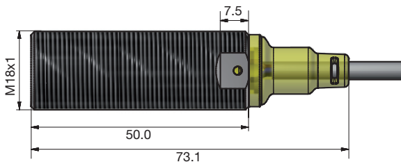
Fig. 26 Long body, flush version, cable
